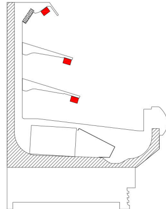
Dairy End Cap
